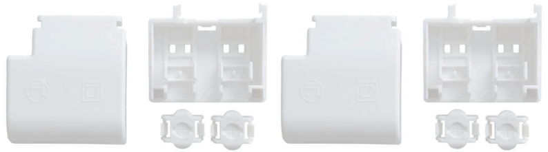
ACU SC 30x43x30mm CLIP-ON SR SET ACU SC 30x43x30mm CLIP-ON SR SET 300 (28001168, non-pre-assembled) (28001351, non-pre-assembled, 300 pcs. packaging)
